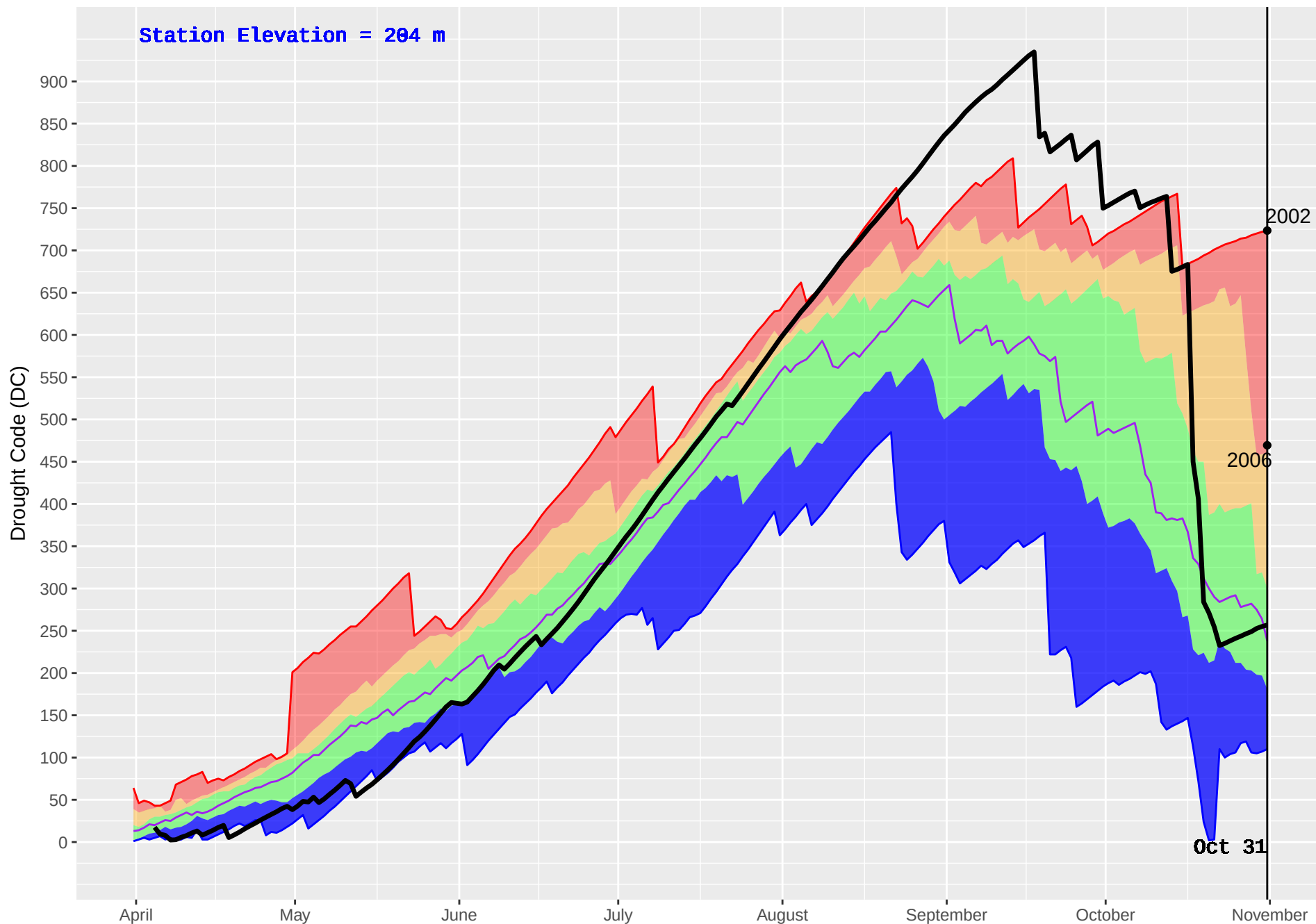
PEMBERTON BASE (301) : Historical (2001–2016) and Current (2017) Noon Drought Code (DC)
