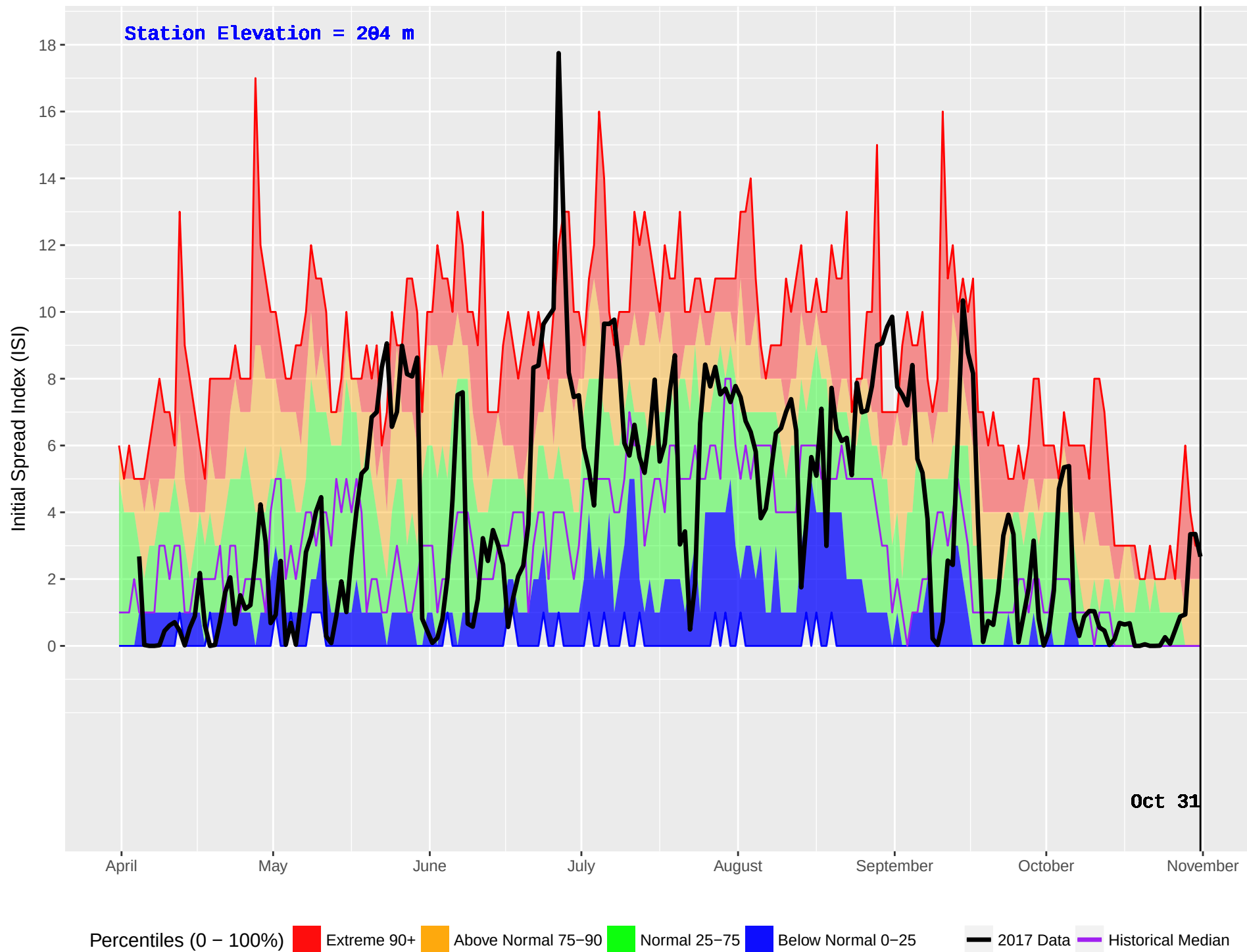
PEMBERTON BASE (301) : Historical (2001–2016) and Current (2017) Noon Initial Spread Index (ISI)
